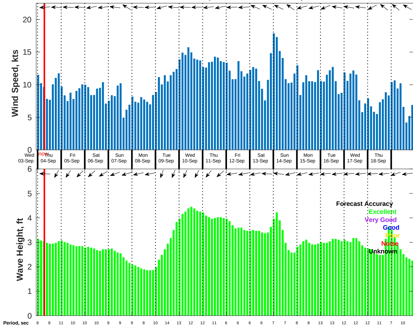
Wind & Wave Forecast for NDBC 52211 from 03-Sep-2025 23:00:00 to 19-Sep-2025 23:00:00
