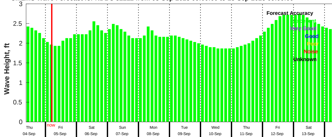
CMEMS Wave Forecast for NDBC 52212 from 03-Sep-2025 09:00:00 to 13-Sep-2025 09:00:00
