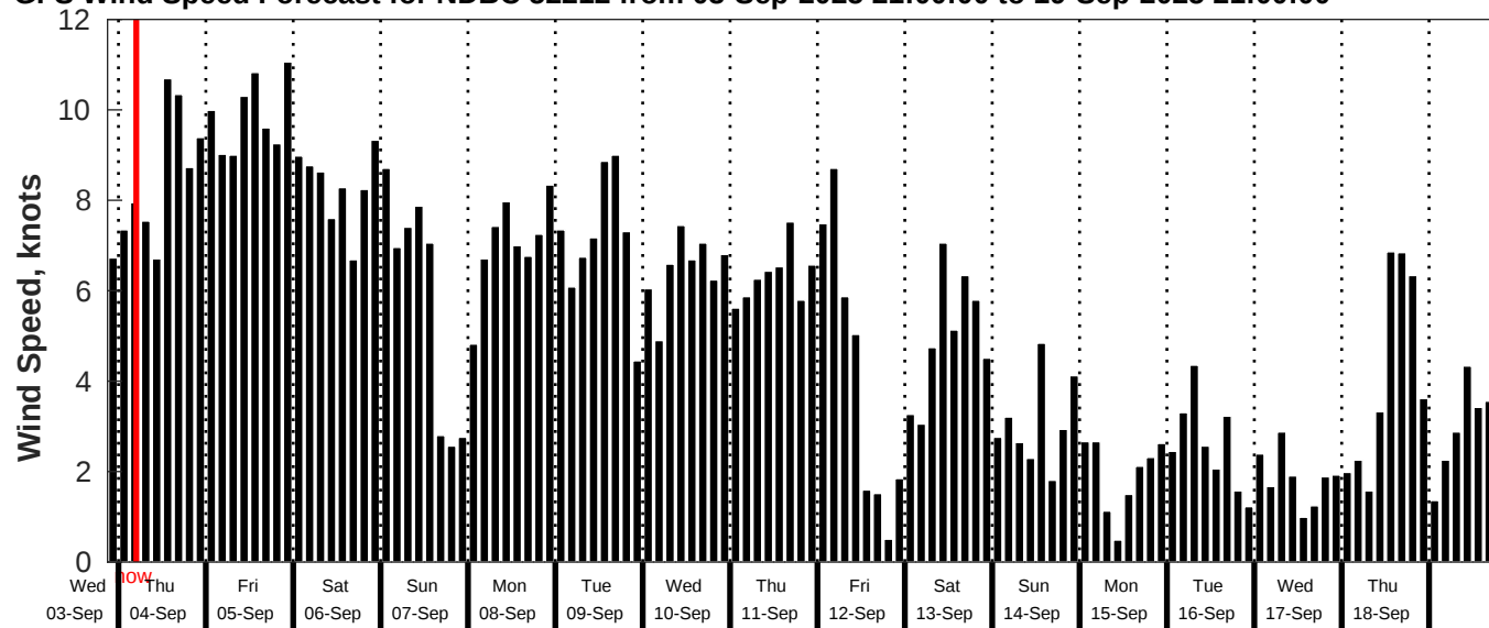
GFS Wind Speed Forecast for NDBC 52212 from 03-Sep-2025 21:00:00 to 19-Sep-2025 21:00:00
