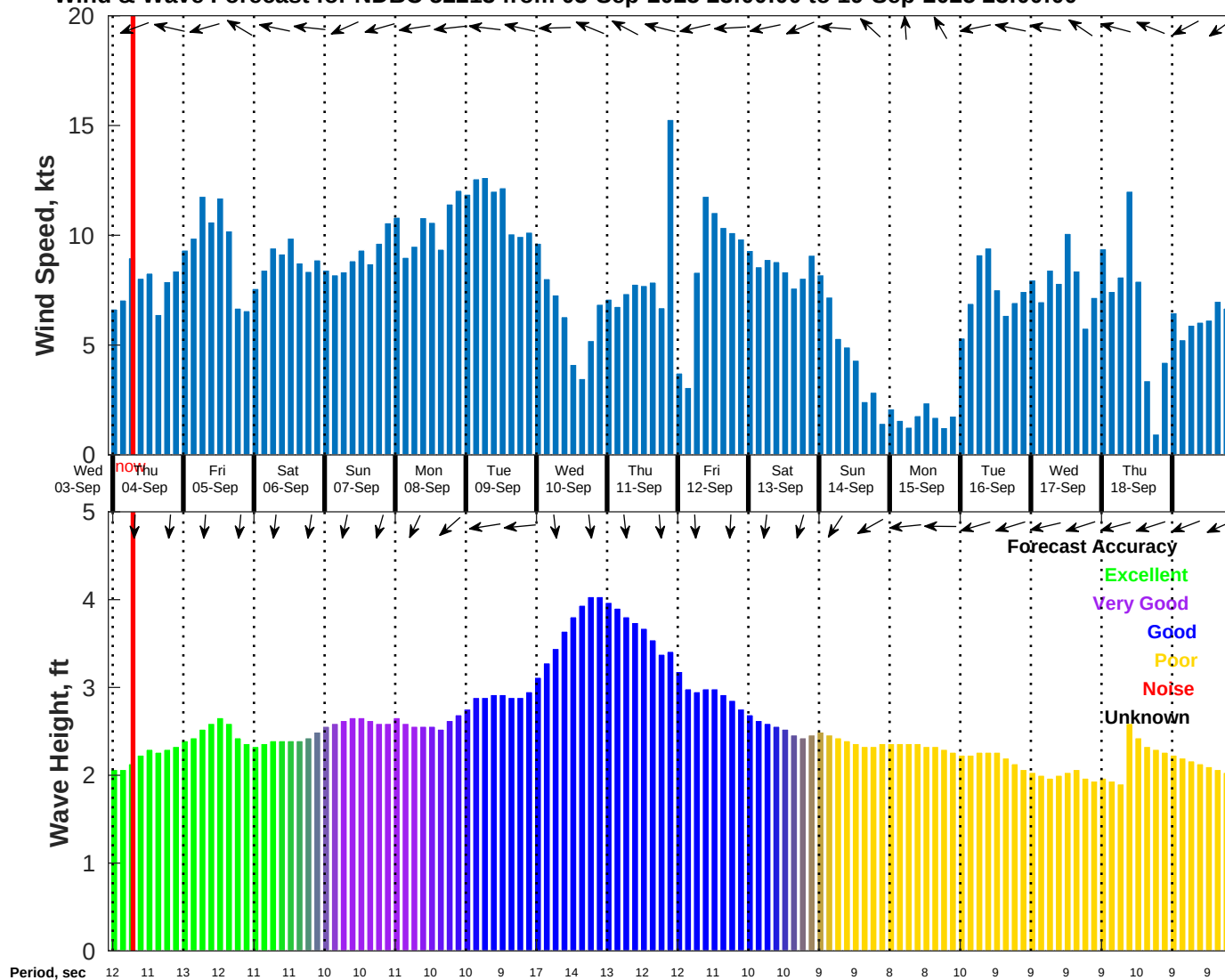
Wind & Wave Forecast for NDBC 52213 from 03-Sep-2025 23:00:00 to 19-Sep-2025 23:00:00
