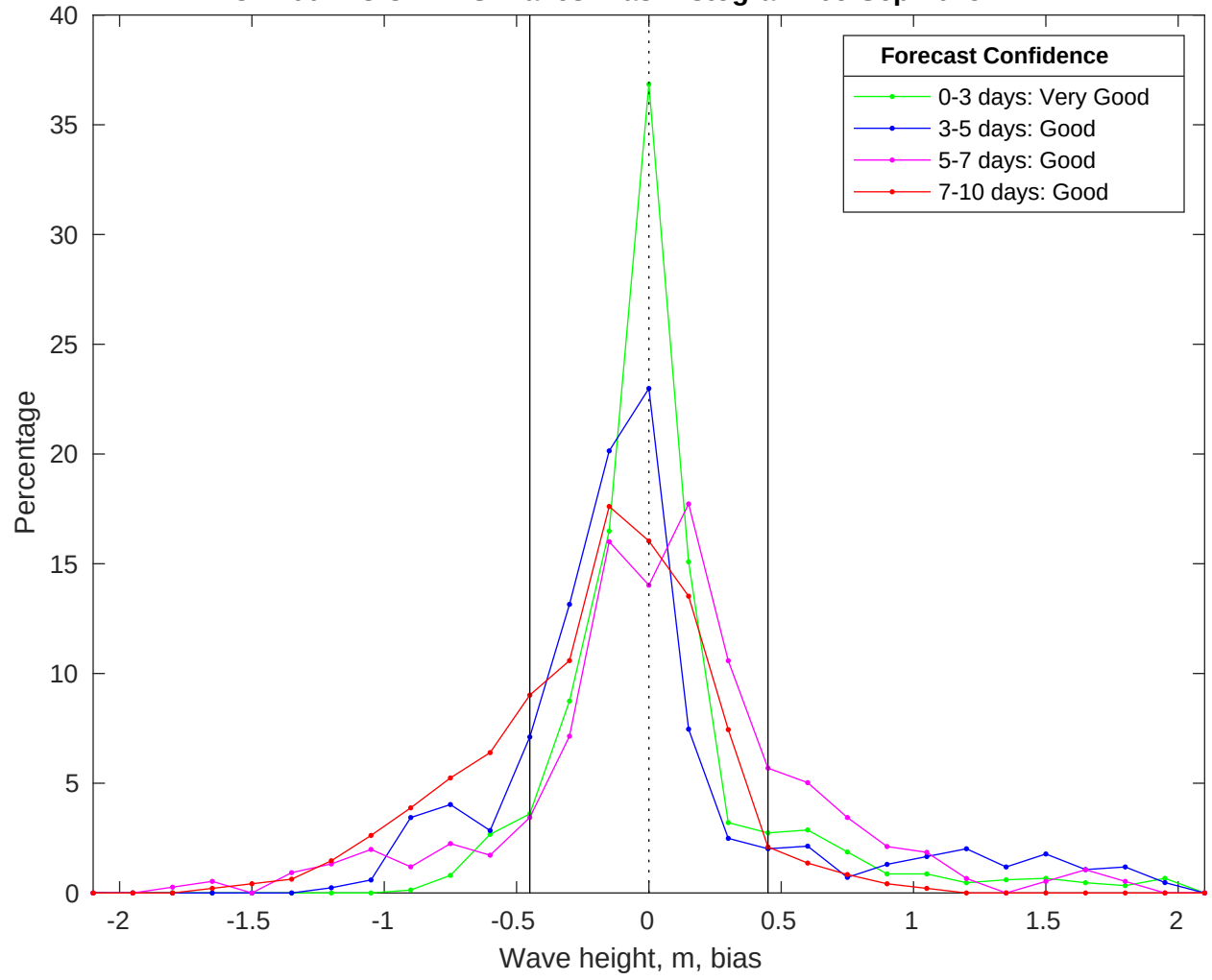
NDBC 41004 vs CMEMS Waves Bias Histogram: 05-Sep-2025
