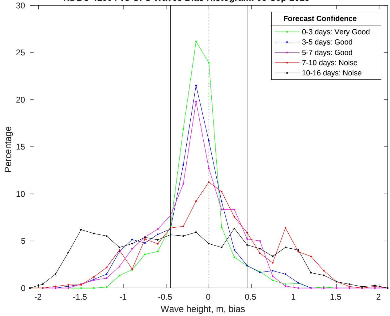
NDBC 41004 vs GFS Waves Bias Histogram: 05-Sep-2025
