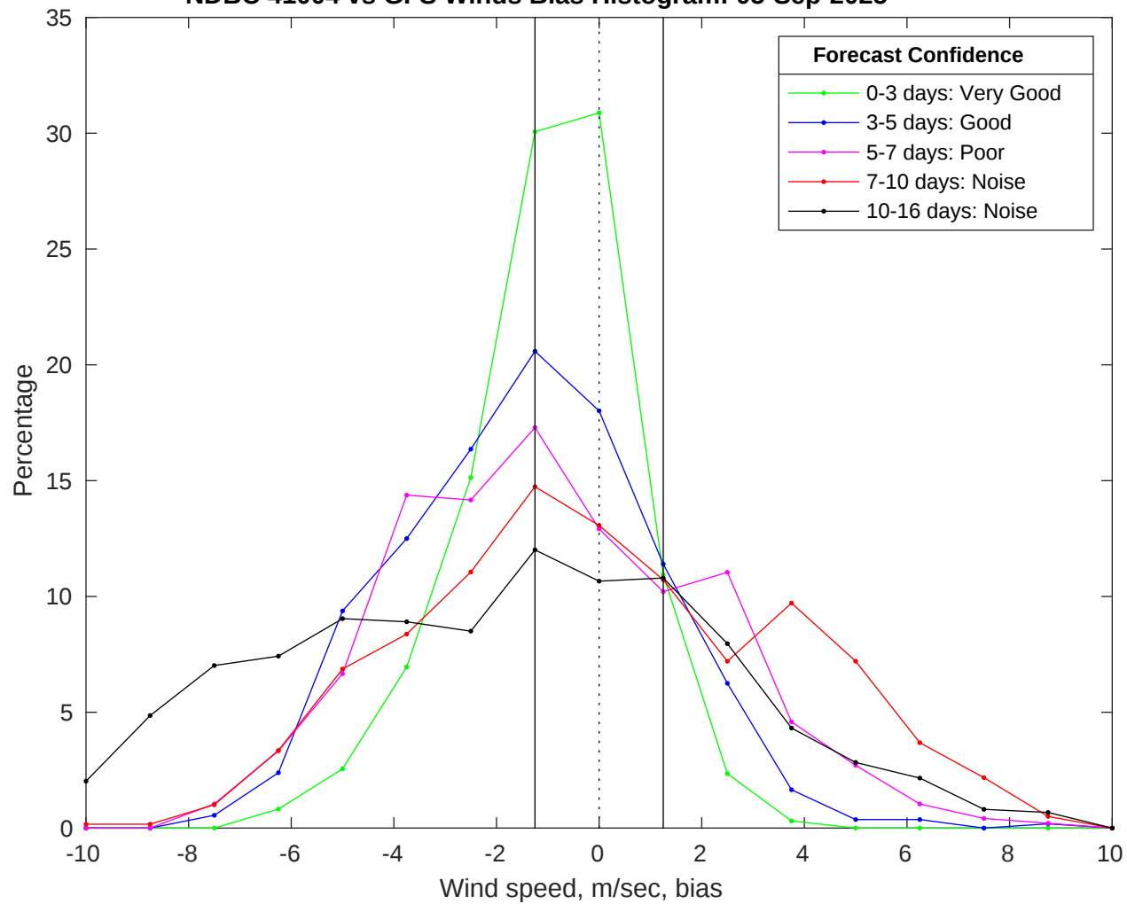
NDBC 41004 vs GFS Winds Bias Histogram: 05-Sep-2025
