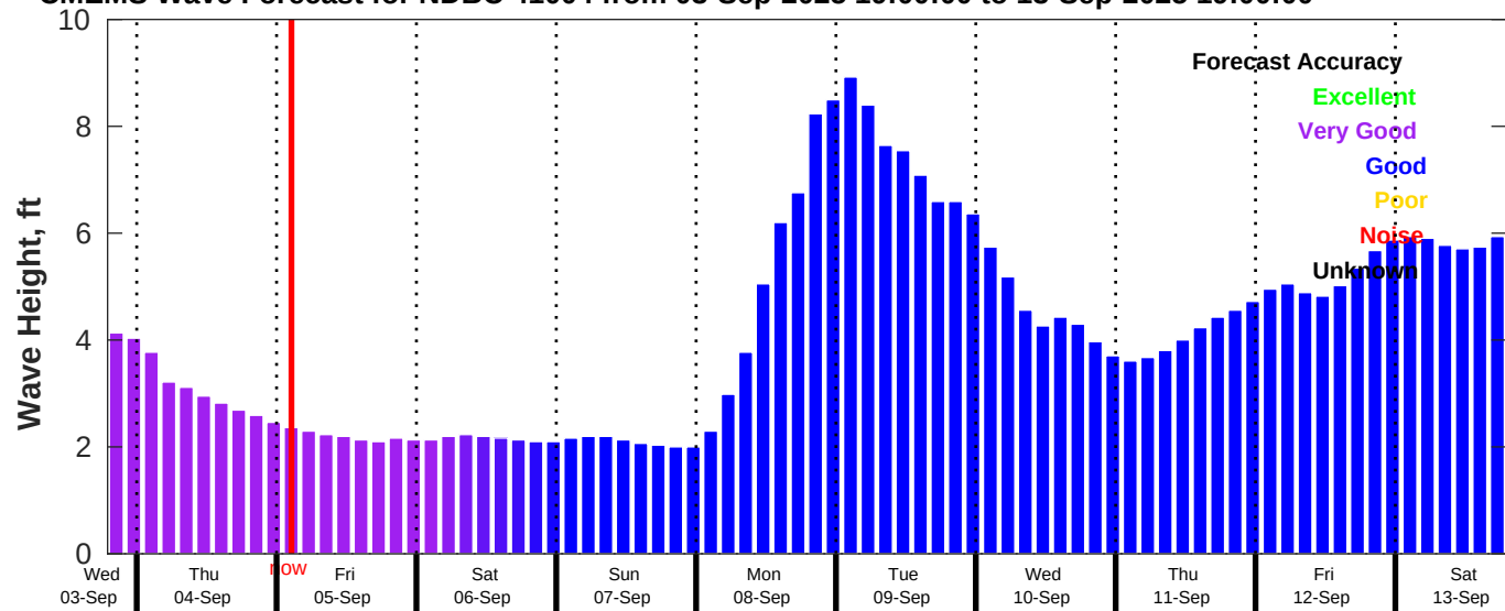
CMEMS Wave Forecast for NDBC 41004 from 03-Sep-2025 19:00:00 to 13-Sep-2025 19:00:00
