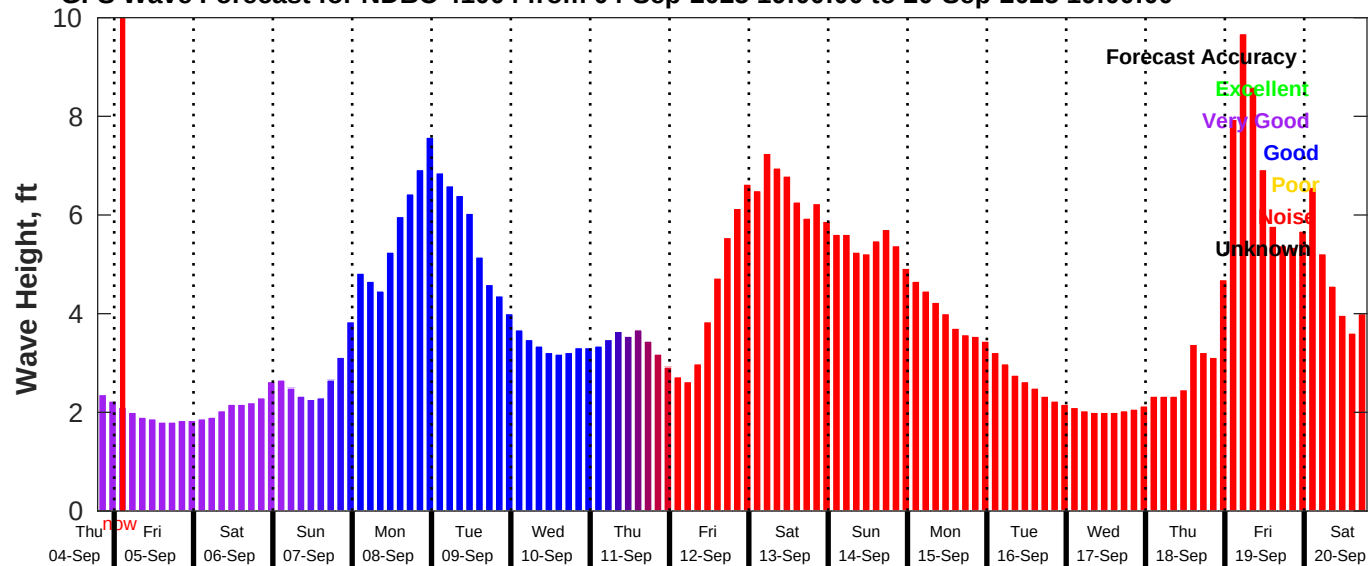
GFS Wave Forecast for NDBC 41004 from 04-Sep-2025 19:00:00 to 20-Sep-2025 19:00:00
