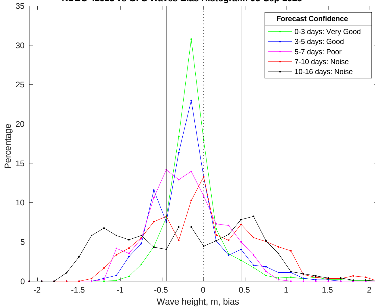
NDBC 41013 vs GFS Waves Bias Histogram: 05-Sep-2025
