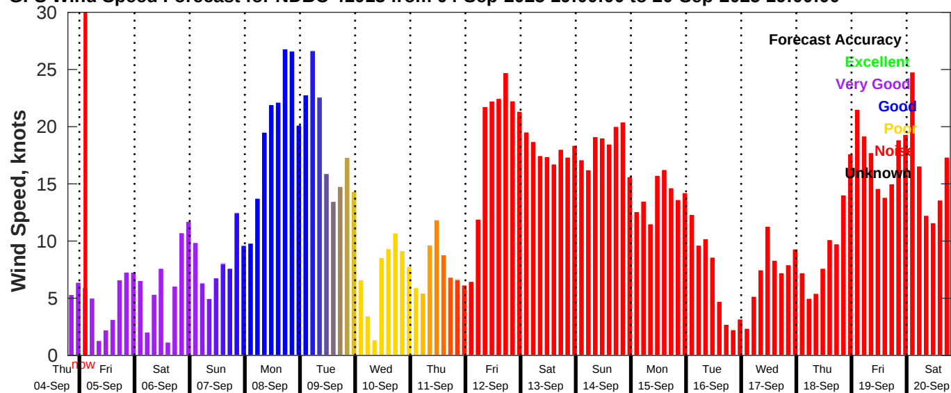
GFS Wind Speed Forecast for NDBC 41013 from 04-Sep-2025 19:00:00 to 20-Sep-2025 19:00:00
