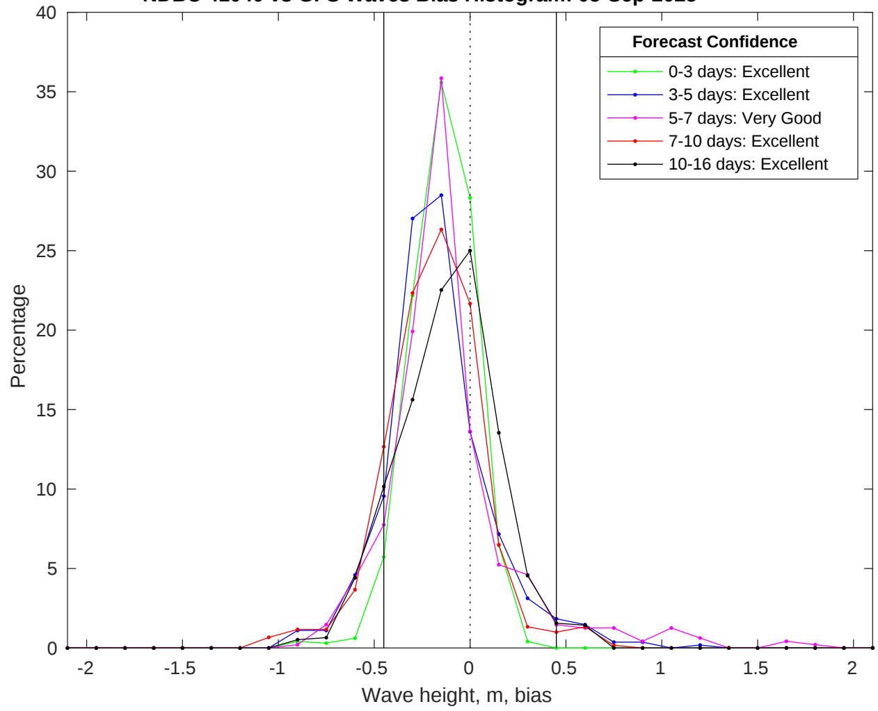
NDBC 41040 vs GFS Waves Bias Histogram: 05-Sep-2025
