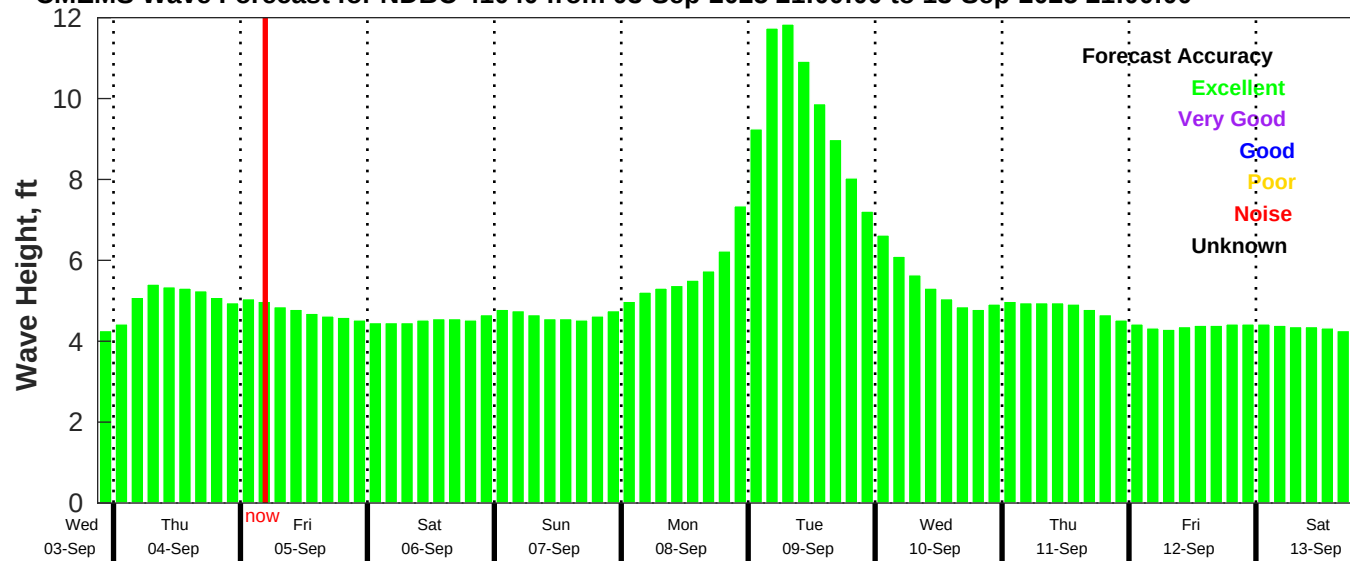
CMEMS Wave Forecast for NDBC 41040 from 03-Sep-2025 21:00:00 to 13-Sep-2025 21:00:00
