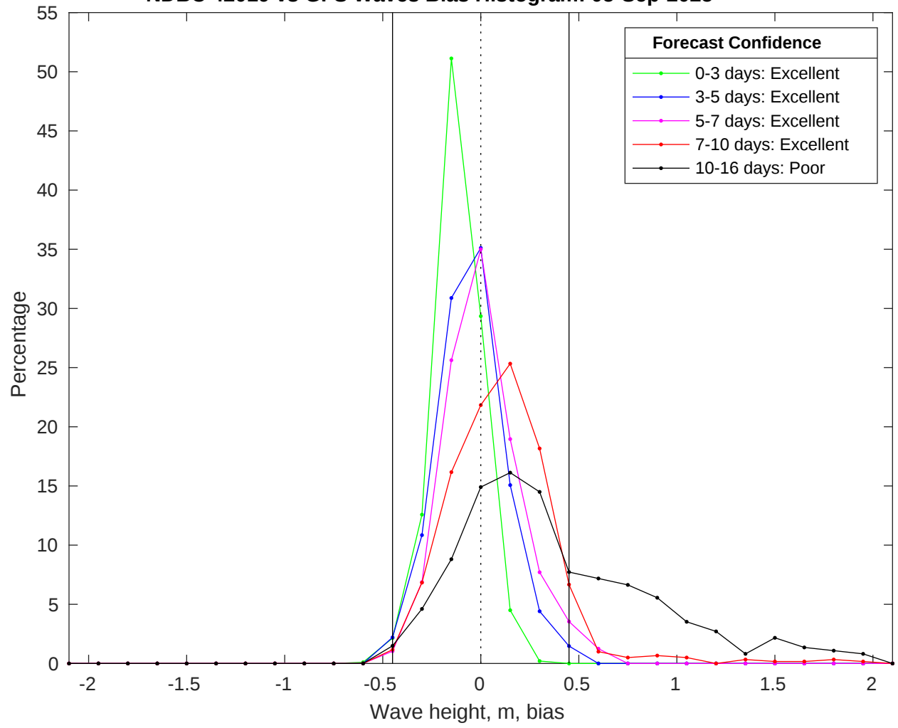
NDBC 42019 vs GFS Waves Bias Histogram: 05-Sep-2025
