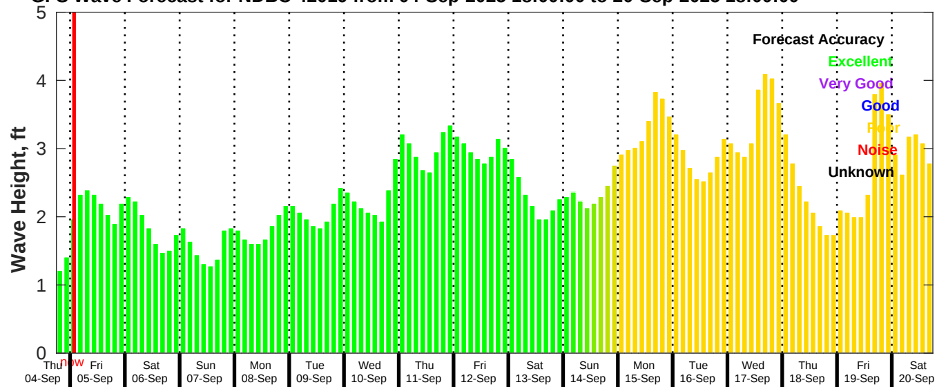
GFS Wave Forecast for NDBC 42019 from 04-Sep-2025 18:00:00 to 20-Sep-2025 18:00:00
