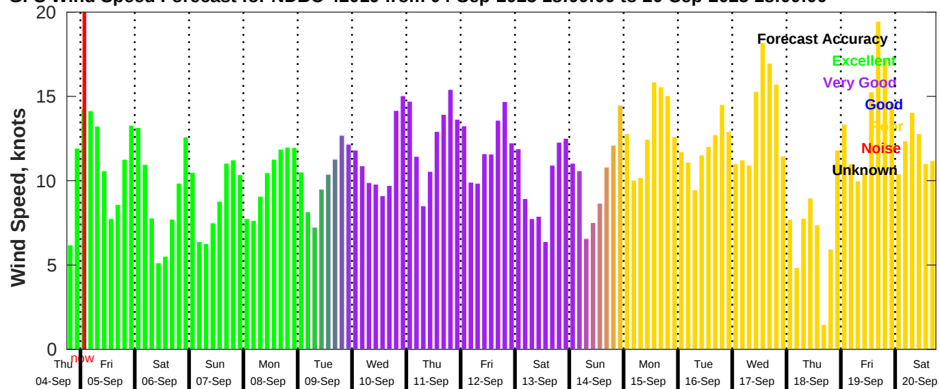
GFS Wind Speed Forecast for NDBC 42019 from 04-Sep-2025 18:00:00 to 20-Sep-2025 18:00:00
