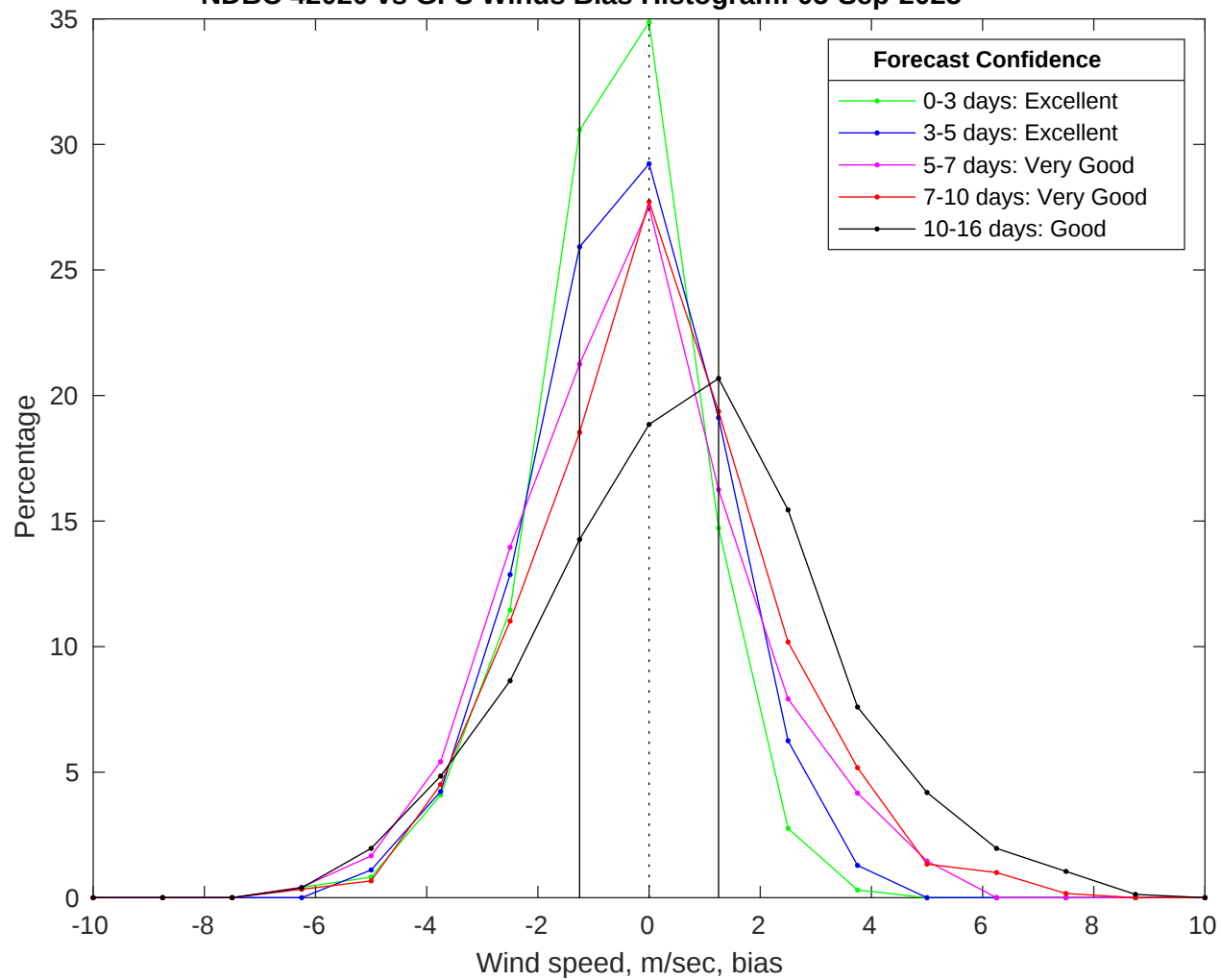
NDBC 42020 vs GFS Winds Bias Histogram: 05-Sep-2025
