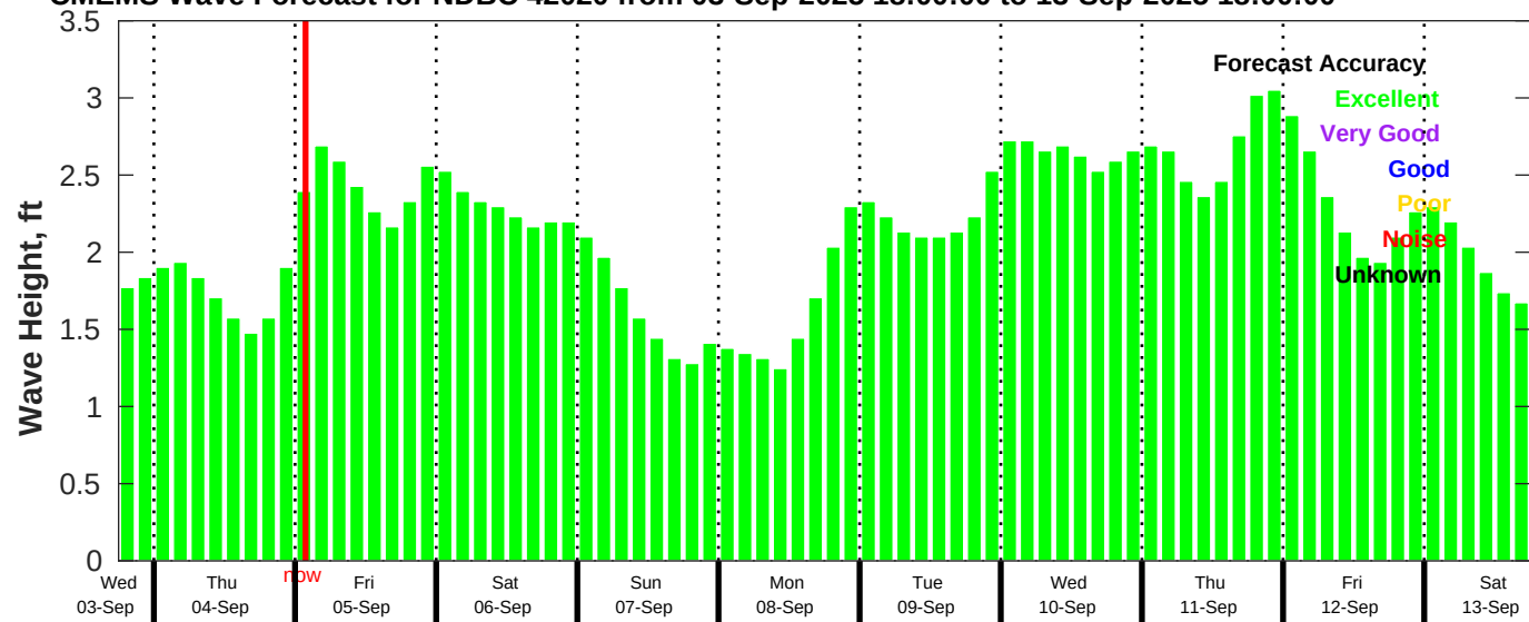
CMEMS Wave Forecast for NDBC 42020 from 03-Sep-2025 18:00:00 to 13-Sep-2025 18:00:00
