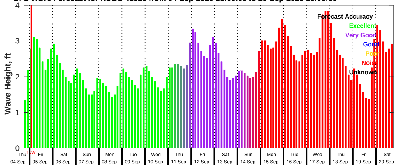
GFS Wave Forecast for NDBC 42020 from 04-Sep-2025 18:00:00 to 20-Sep-2025 18:00:00
