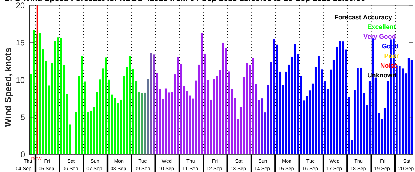
GFS Wind Speed Forecast for NDBC 42020 from 04-Sep-2025 18:00:00 to 20-Sep-2025 18:00:00
