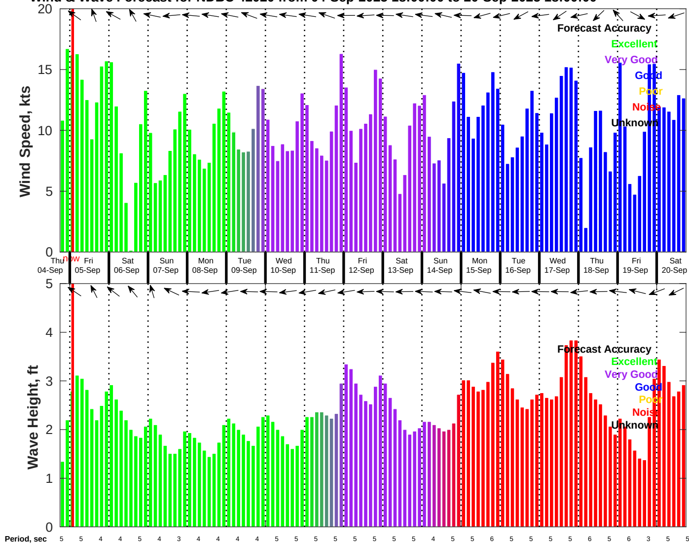
Wind & Wave Forecast for NDBC 42020 from 04-Sep-2025 18:00:00 to 20-Sep-2025 18:00:00
