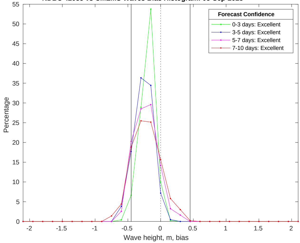
NDBC 42035 vs CMEMS Waves Bias Histogram: 05-Sep-2025
