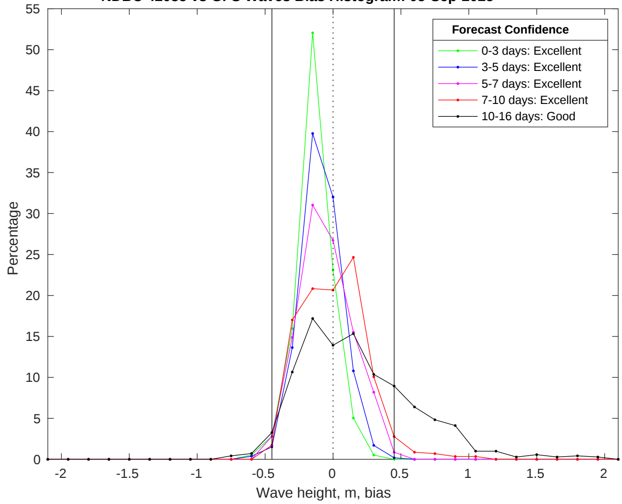
NDBC 42035 vs GFS Waves Bias Histogram: 05-Sep-2025
