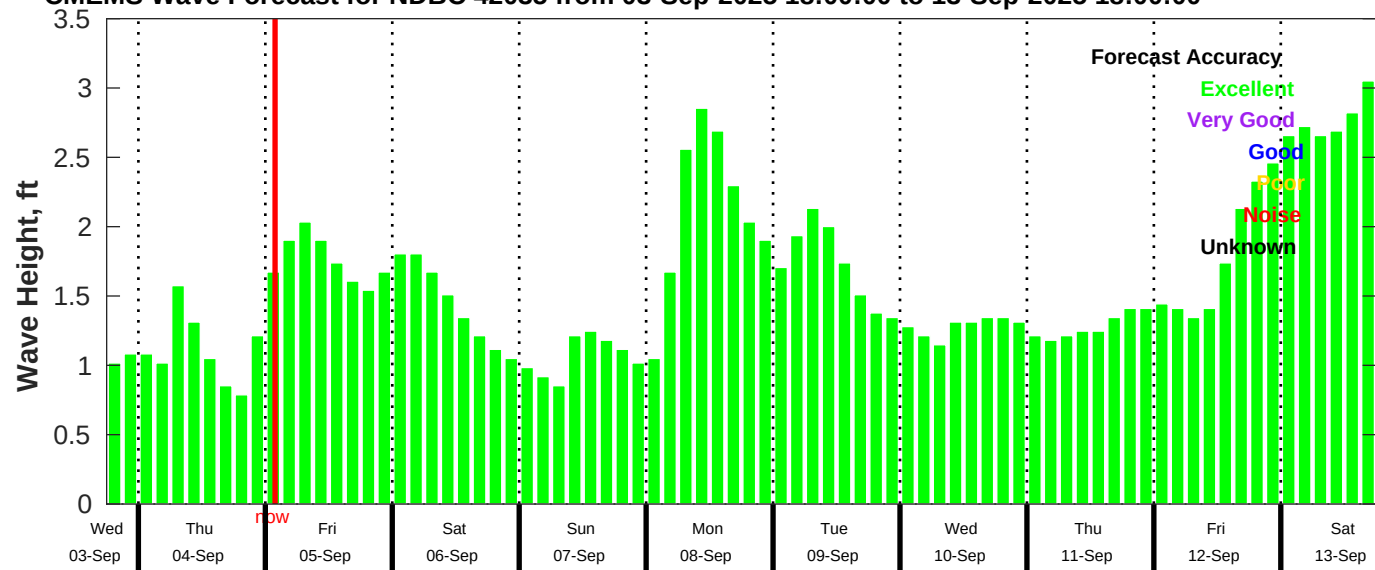
CMEMS Wave Forecast for NDBC 42035 from 03-Sep-2025 18:00:00 to 13-Sep-2025 18:00:00
