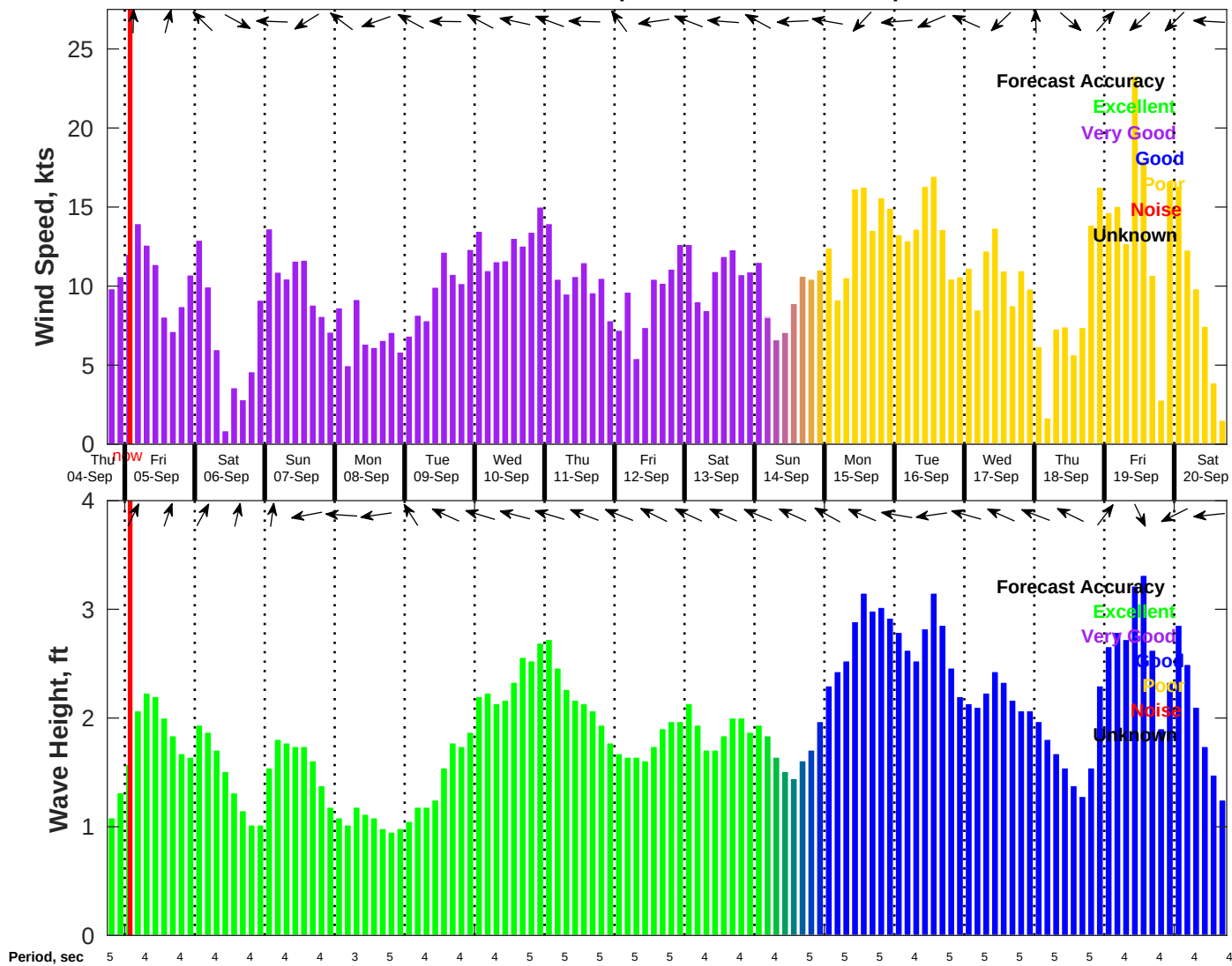
Wind & Wave Forecast for NDBC 42035 from 04-Sep-2025 18:00:00 to 20-Sep-2025 18:00:00
