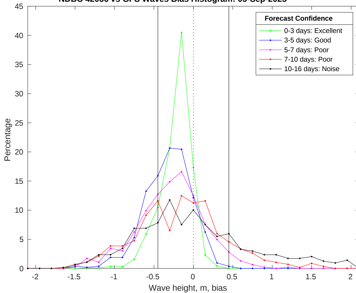
NDBC 42036 vs GFS Waves Bias Histogram: 05-Sep-2025
