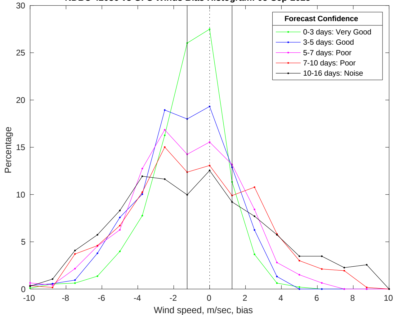
NDBC 42036 vs GFS Winds Bias Histogram: 05-Sep-2025
