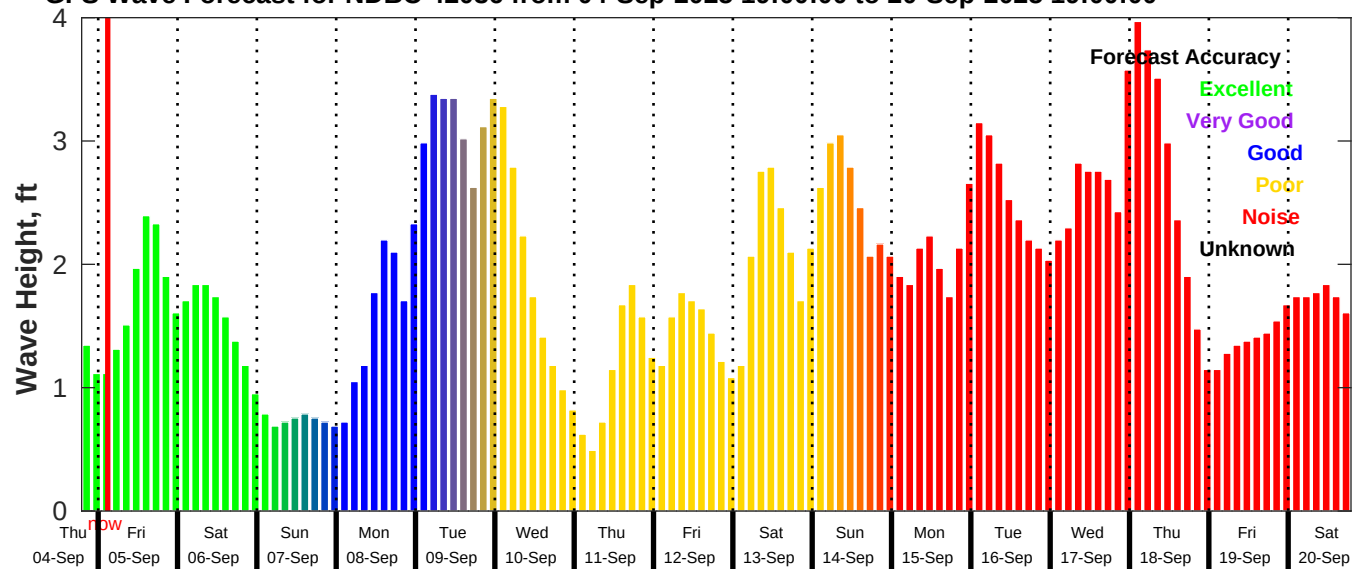
GFS Wave Forecast for NDBC 42036 from 04-Sep-2025 19:00:00 to 20-Sep-2025 19:00:00
