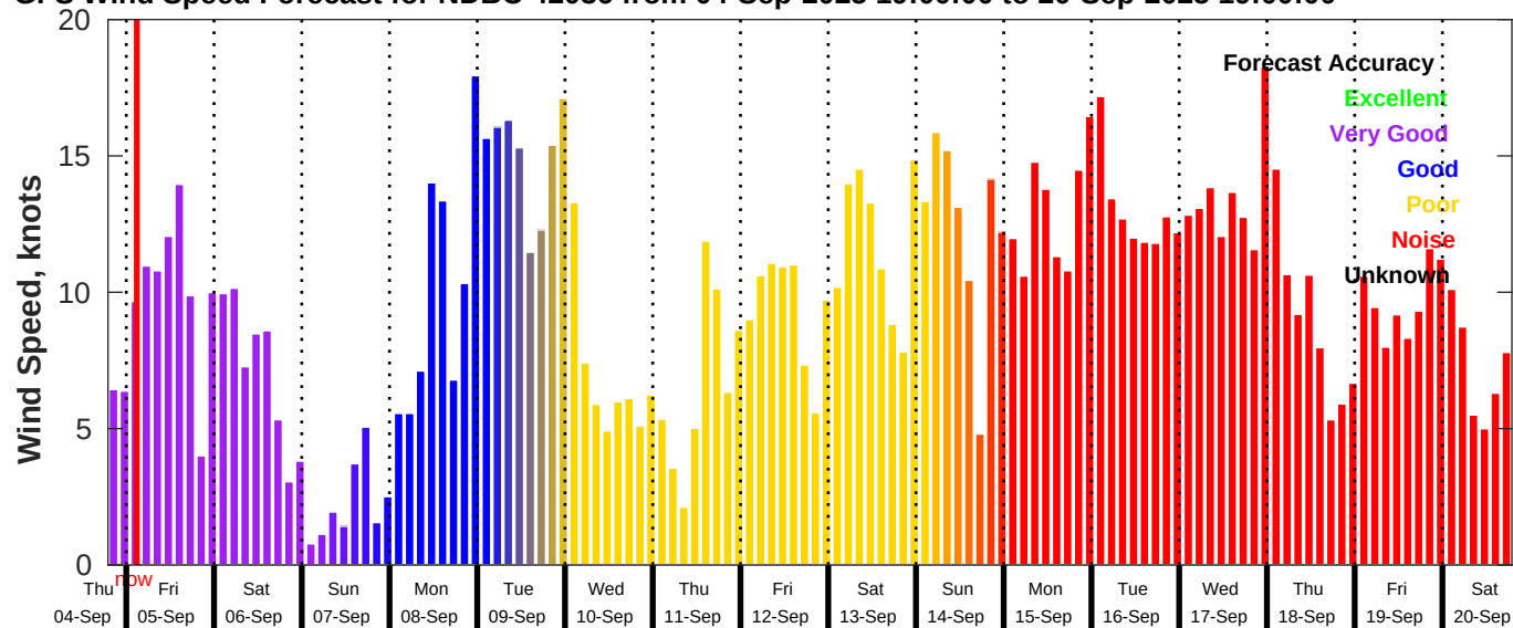
GFS Wind Speed Forecast for NDBC 42036 from 04-Sep-2025 19:00:00 to 20-Sep-2025 19:00:00
