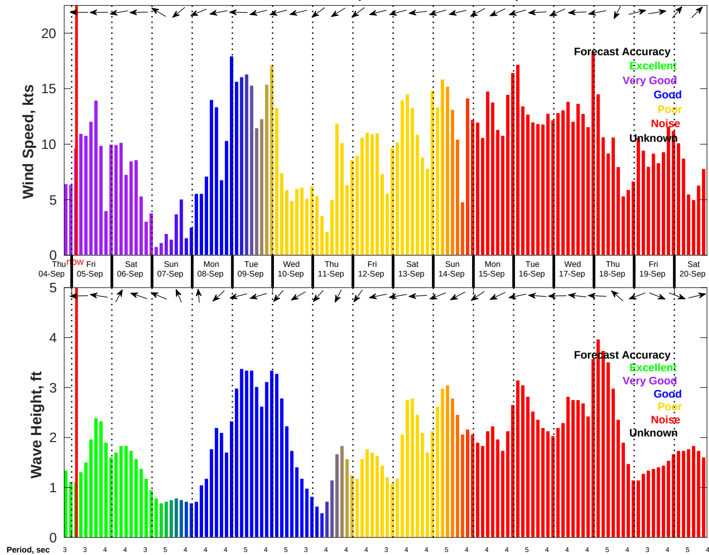
Wind & Wave Forecast for NDBC 42036 from 04-Sep-2025 19:00:00 to 20-Sep-2025 19:00:00
