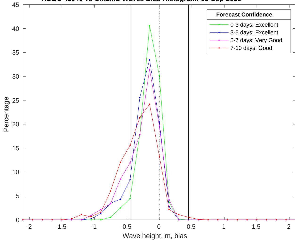
NDBC 42040 vs CMEMS Waves Bias Histogram: 05-Sep-2025
