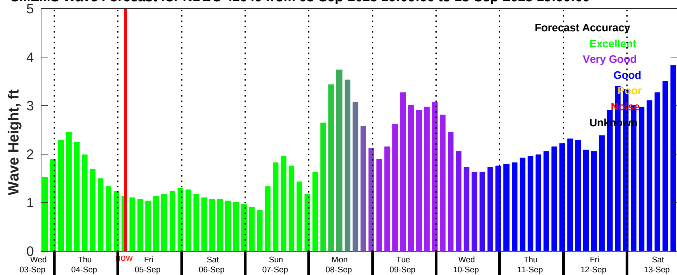
CMEMS Wave Forecast for NDBC 42040 from 03-Sep-2025 19:00:00 to 13-Sep-2025 19:00:00
