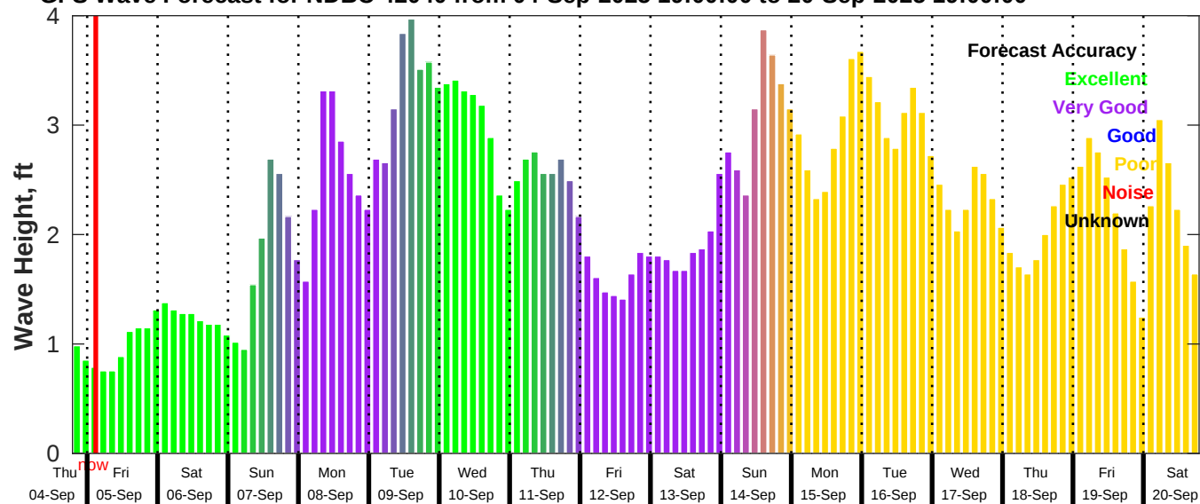
GFS Wave Forecast for NDBC 42040 from 04-Sep-2025 19:00:00 to 20-Sep-2025 19:00:00
