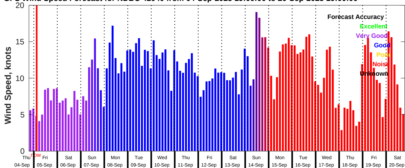
GFS Wind Speed Forecast for NDBC 42040 from 04-Sep-2025 19:00:00 to 20-Sep-2025 19:00:00
