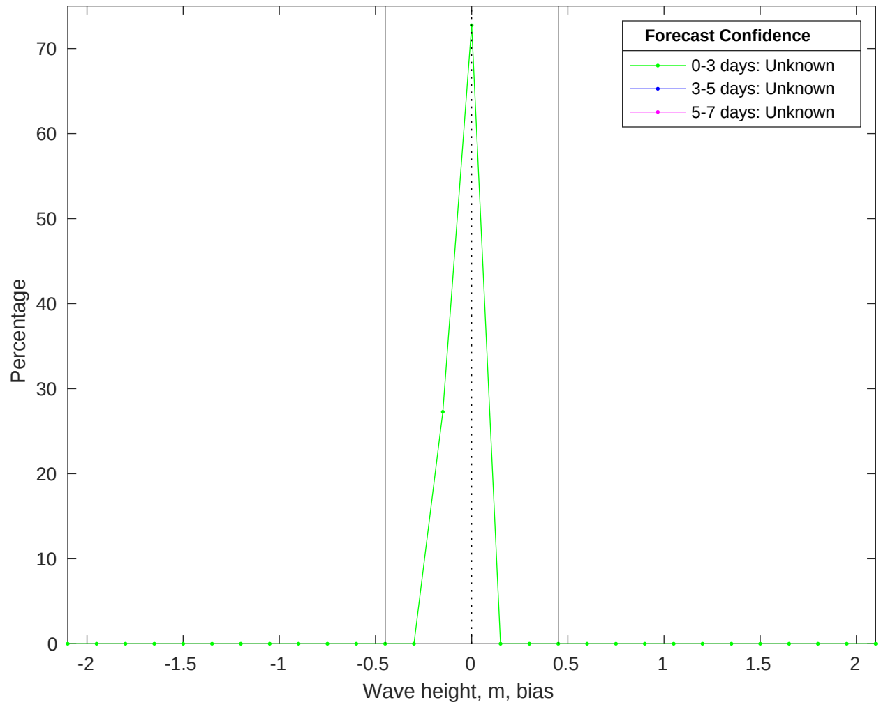
NDBC 44008 vs CMEMS Waves Bias Histogram: 05-Sep-2025
