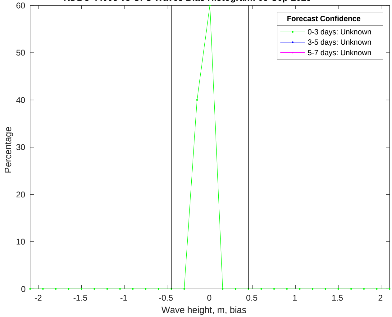
NDBC 44008 vs GFS Waves Bias Histogram: 05-Sep-2025
