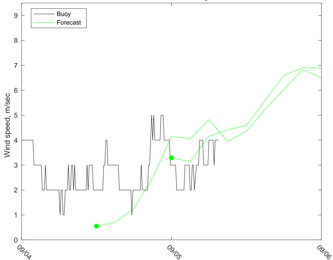
NDBC 44008 vs GFS Winds: 0 to 3 day forecast
