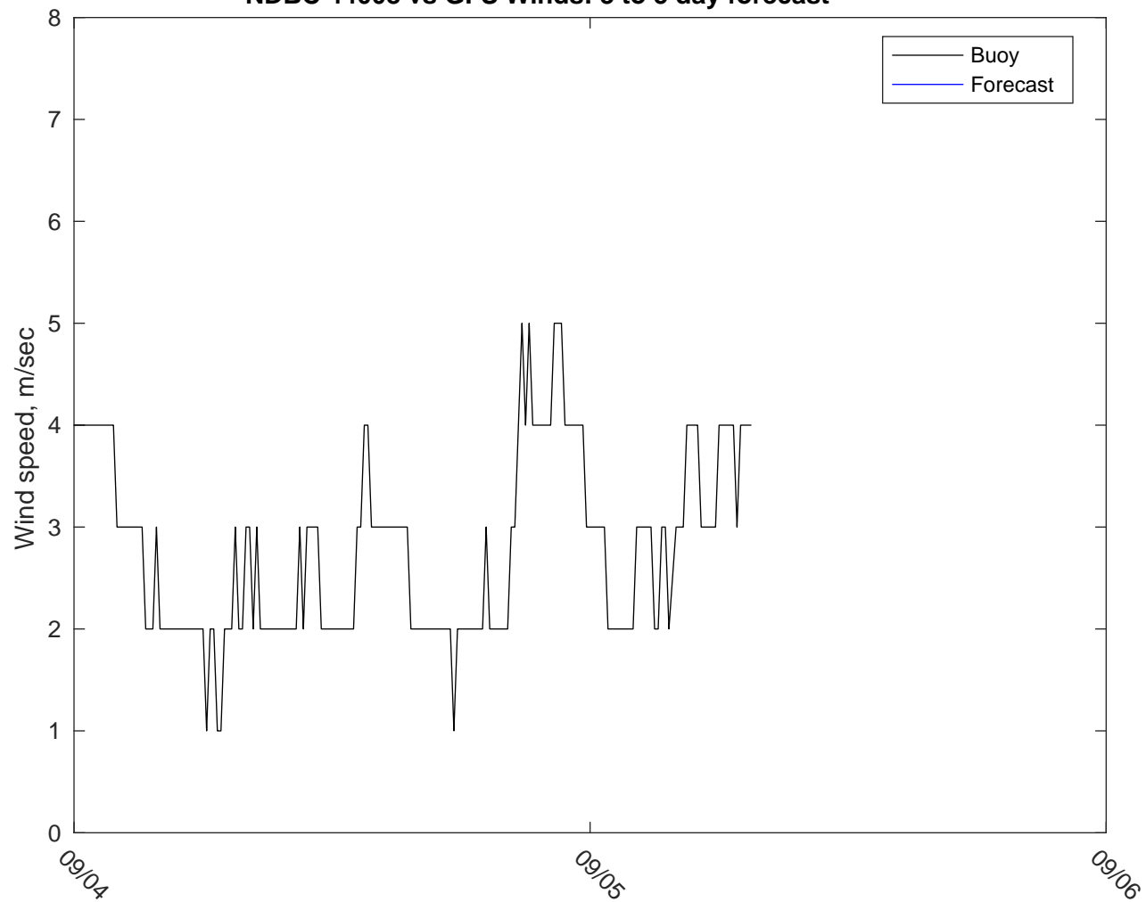
NDBC 44008 vs GFS Winds: 3 to 5 day forecast
