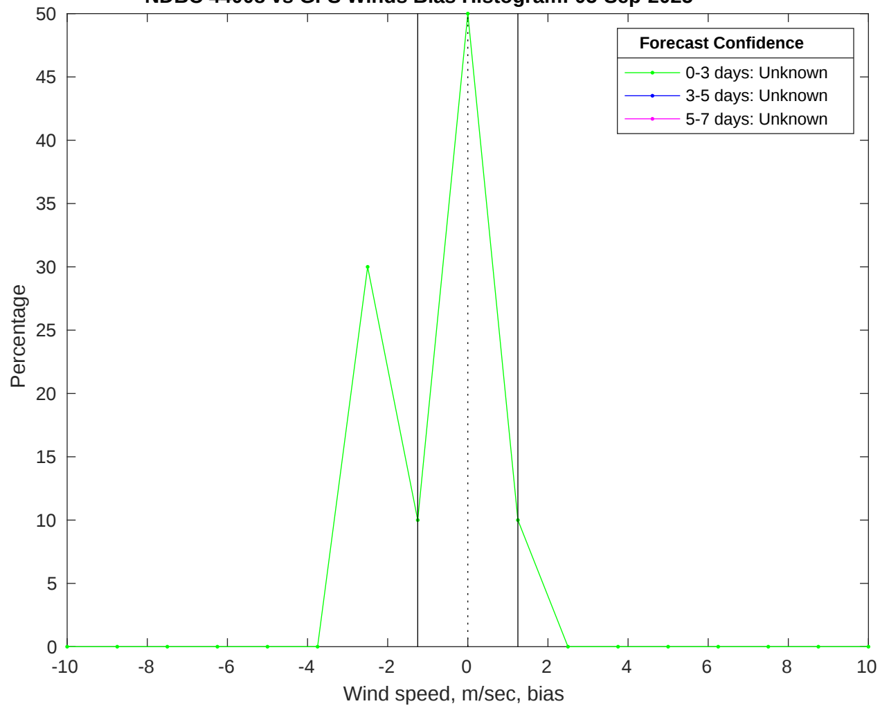
NDBC 44008 vs GFS Winds Bias Histogram: 05-Sep-2025
