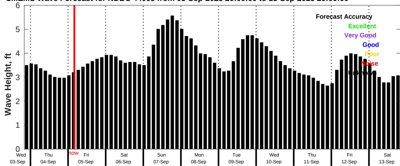
CMEMS Wave Forecast for NDBC 44008 from 03-Sep-2025 20:00:00 to 13-Sep-2025 20:00:00
