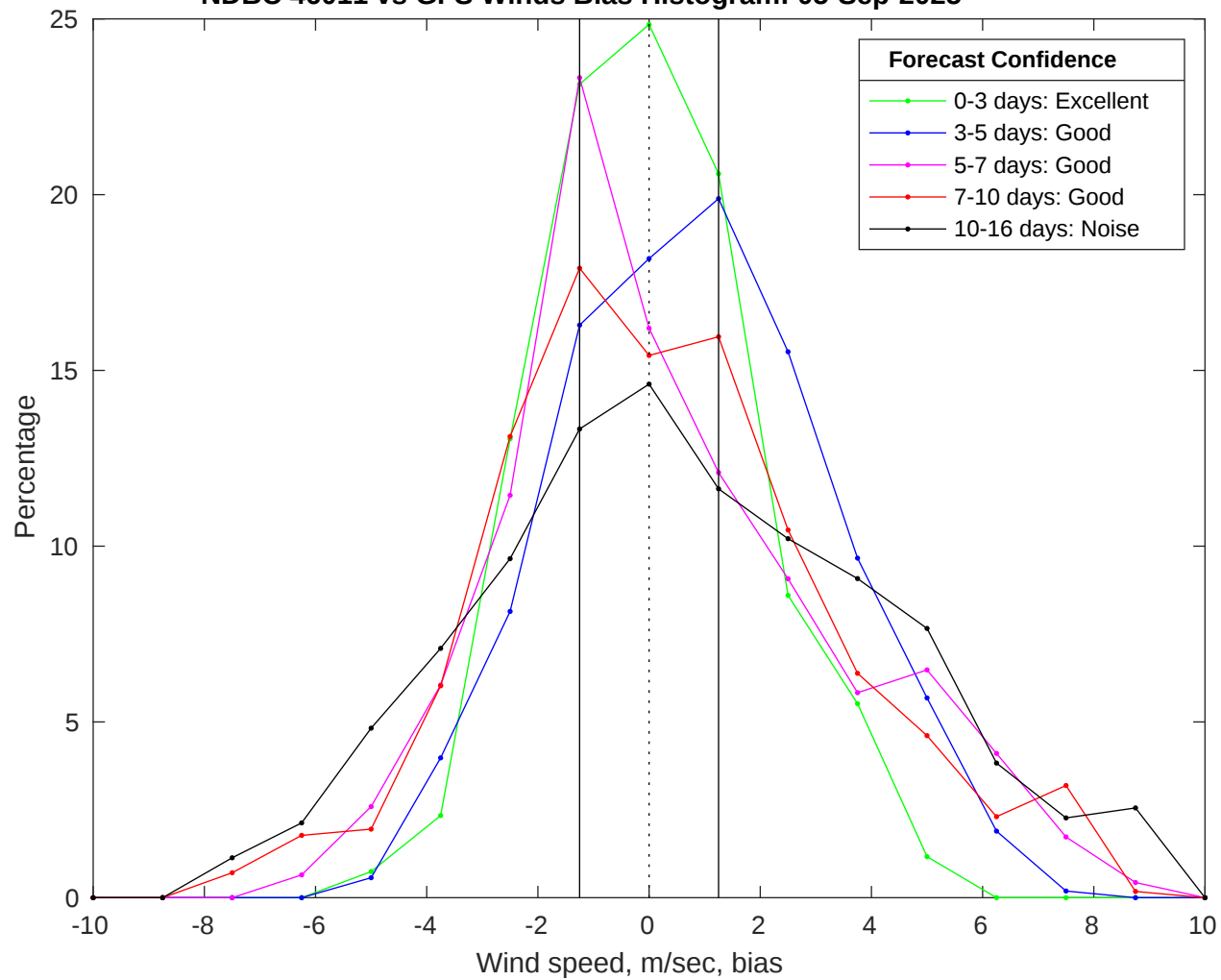
NDBC 46011 vs GFS Winds Bias Histogram: 05-Sep-2025
