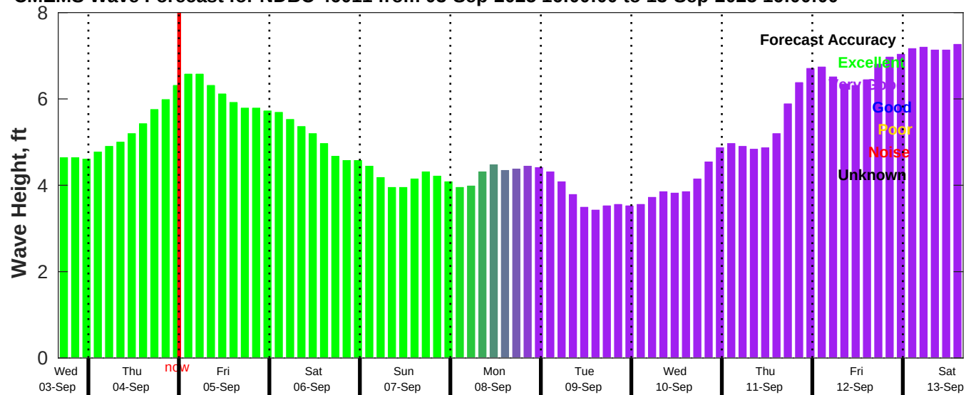
CMEMS Wave Forecast for NDBC 46011 from 03-Sep-2025 16:00:00 to 13-Sep-2025 16:00:00
