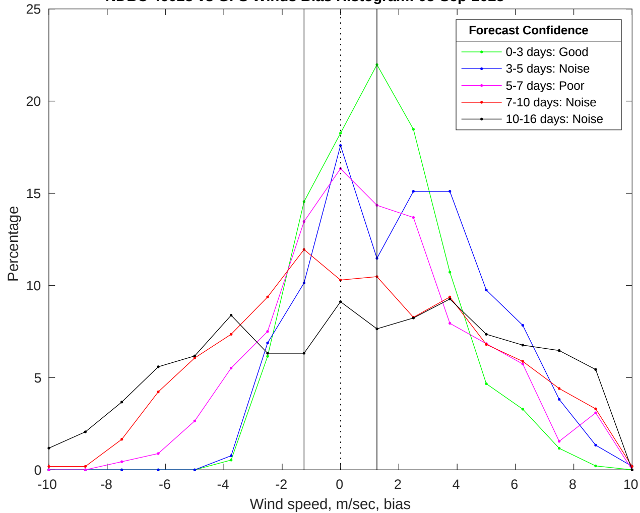
NDBC 46028 vs GFS Winds Bias Histogram: 05-Sep-2025
