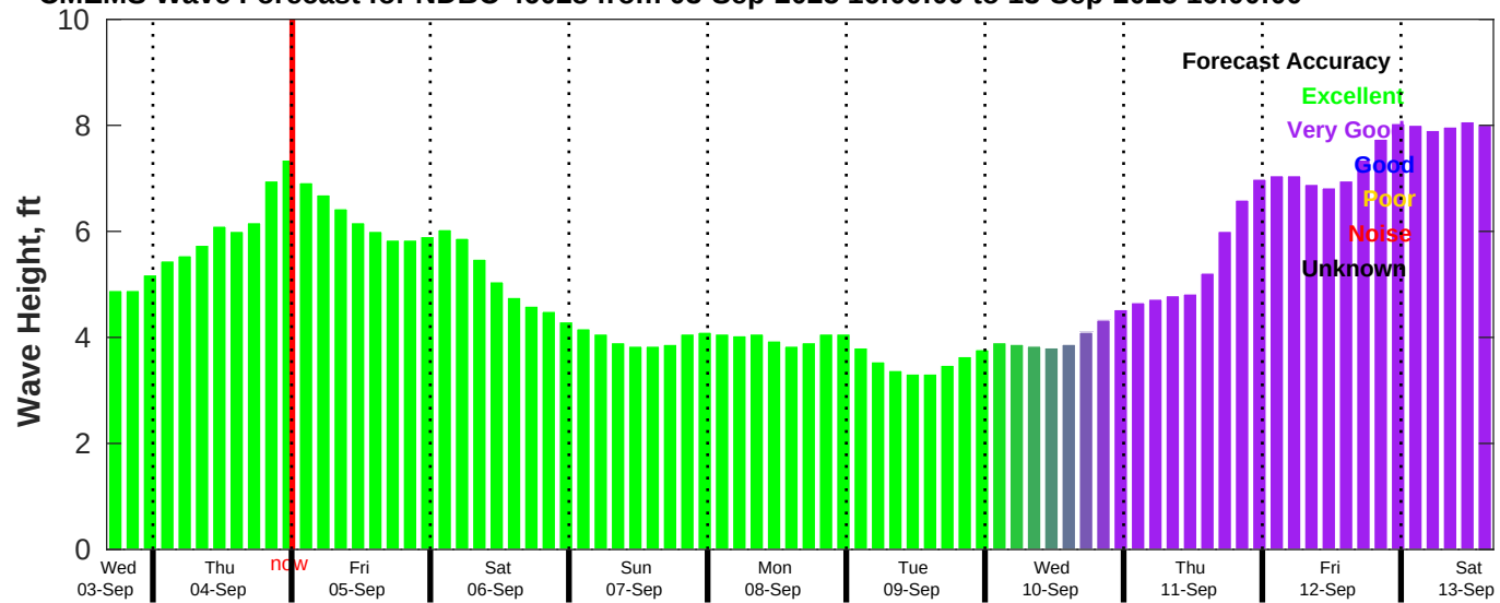
CMEMS Wave Forecast for NDBC 46028 from 03-Sep-2025 16:00:00 to 13-Sep-2025 16:00:00
