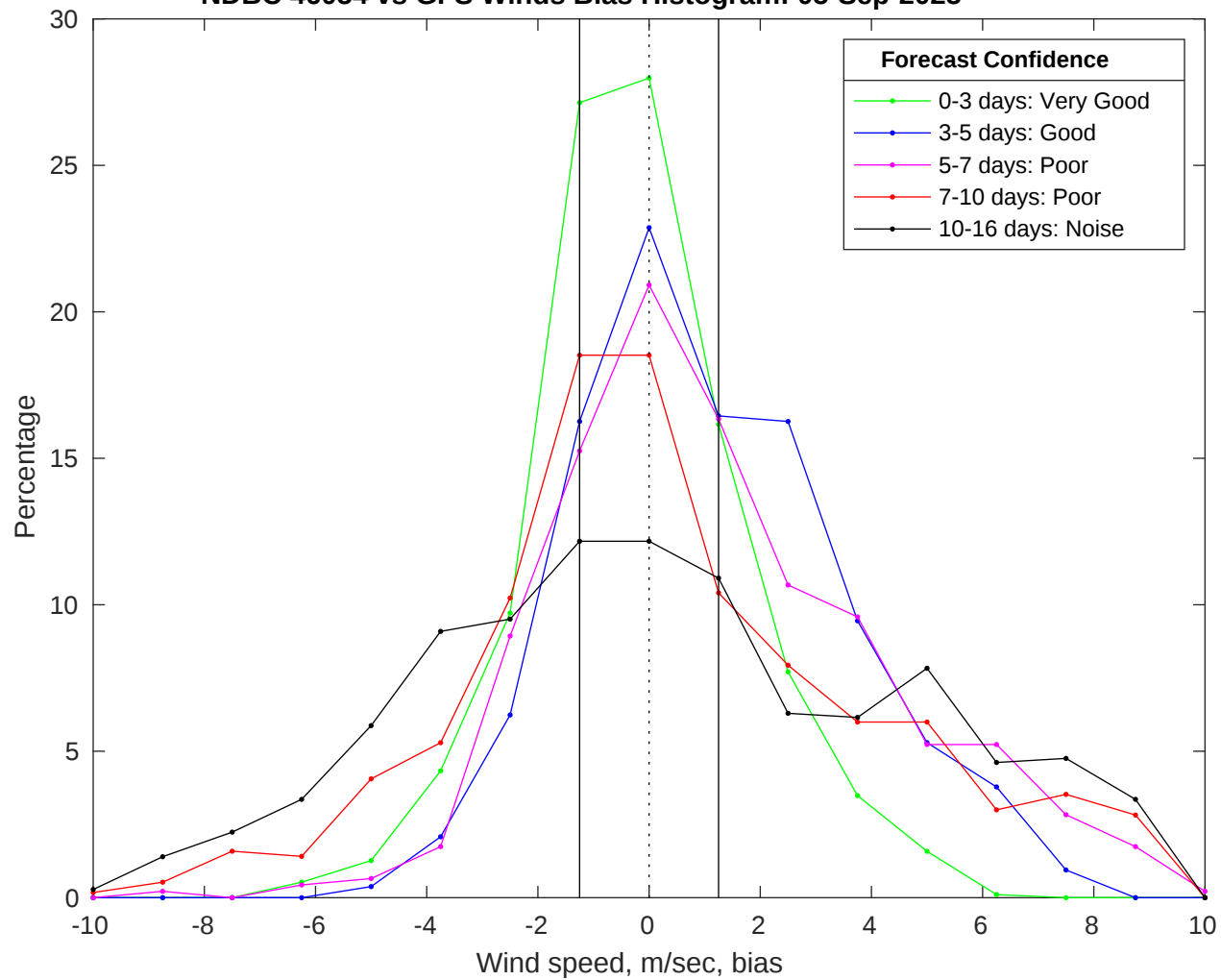
NDBC 46054 vs GFS Winds Bias Histogram: 05-Sep-2025
