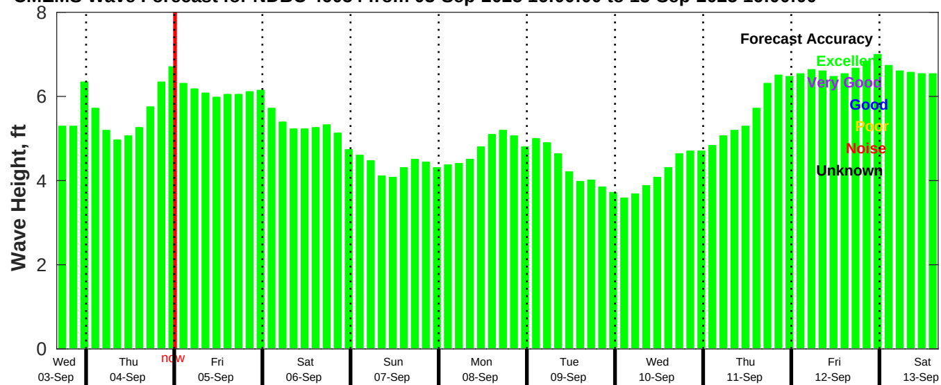
CMEMS Wave Forecast for NDBC 46054 from 03-Sep-2025 16:00:00 to 13-Sep-2025 16:00:00
