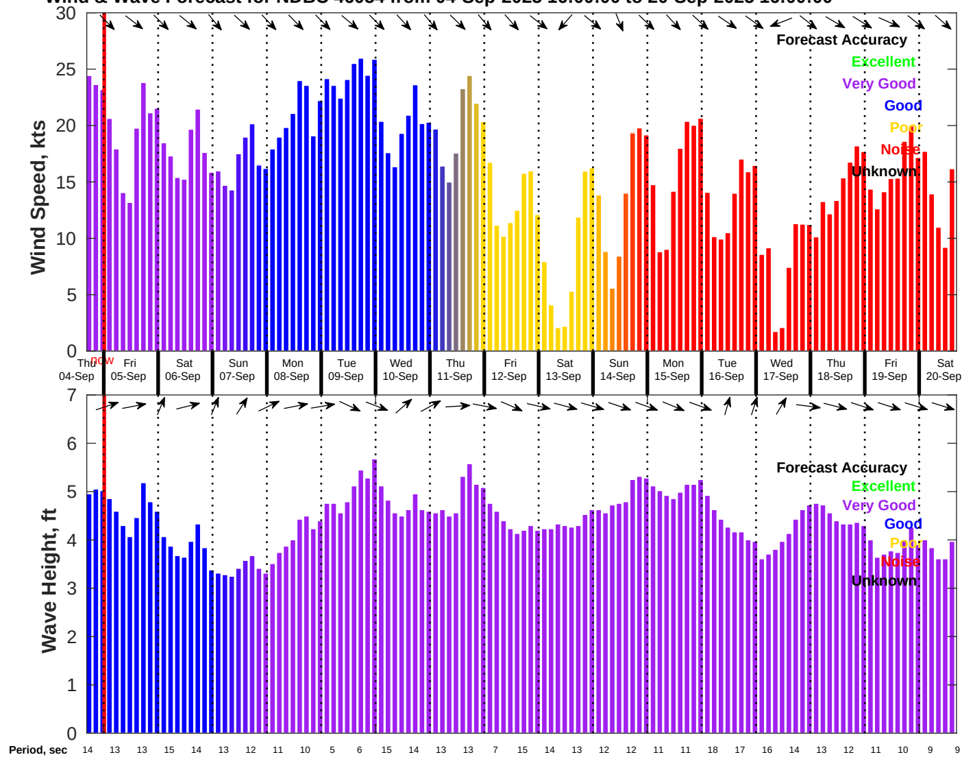
Wind & Wave Forecast for NDBC 46054 from 04-Sep-2025 16:00:00 to 20-Sep-2025 16:00:00
