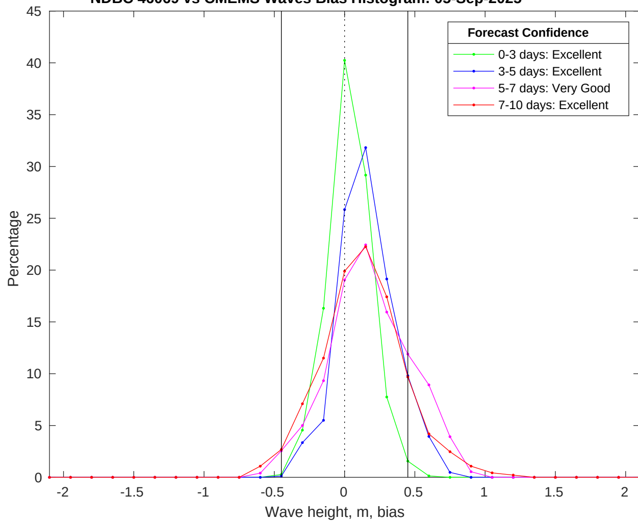
NDBC 46069 vs CMEMS Waves Bias Histogram: 05-Sep-2025
