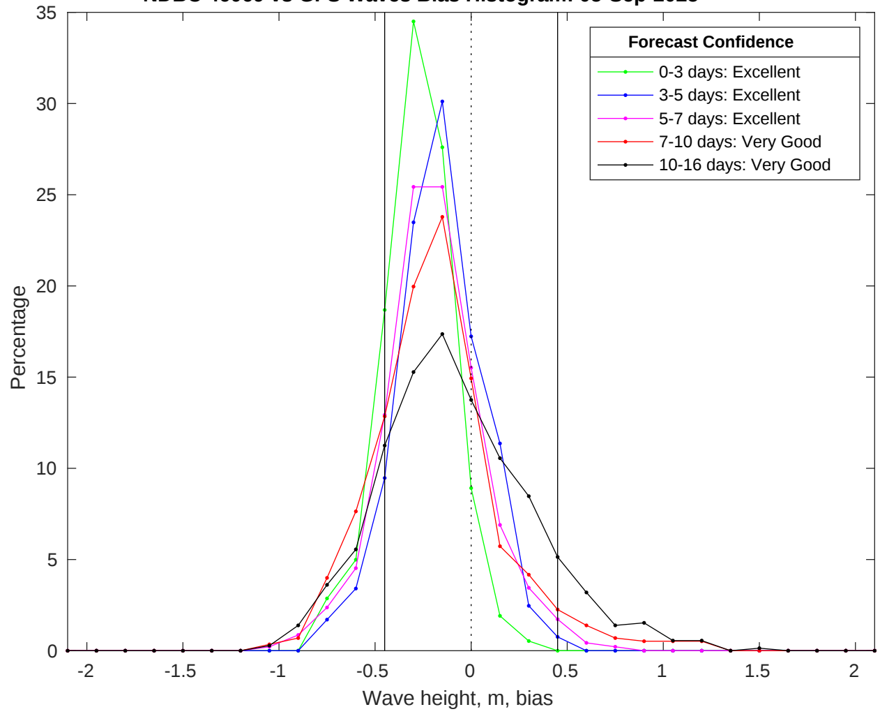
NDBC 46069 vs GFS Waves Bias Histogram: 05-Sep-2025
