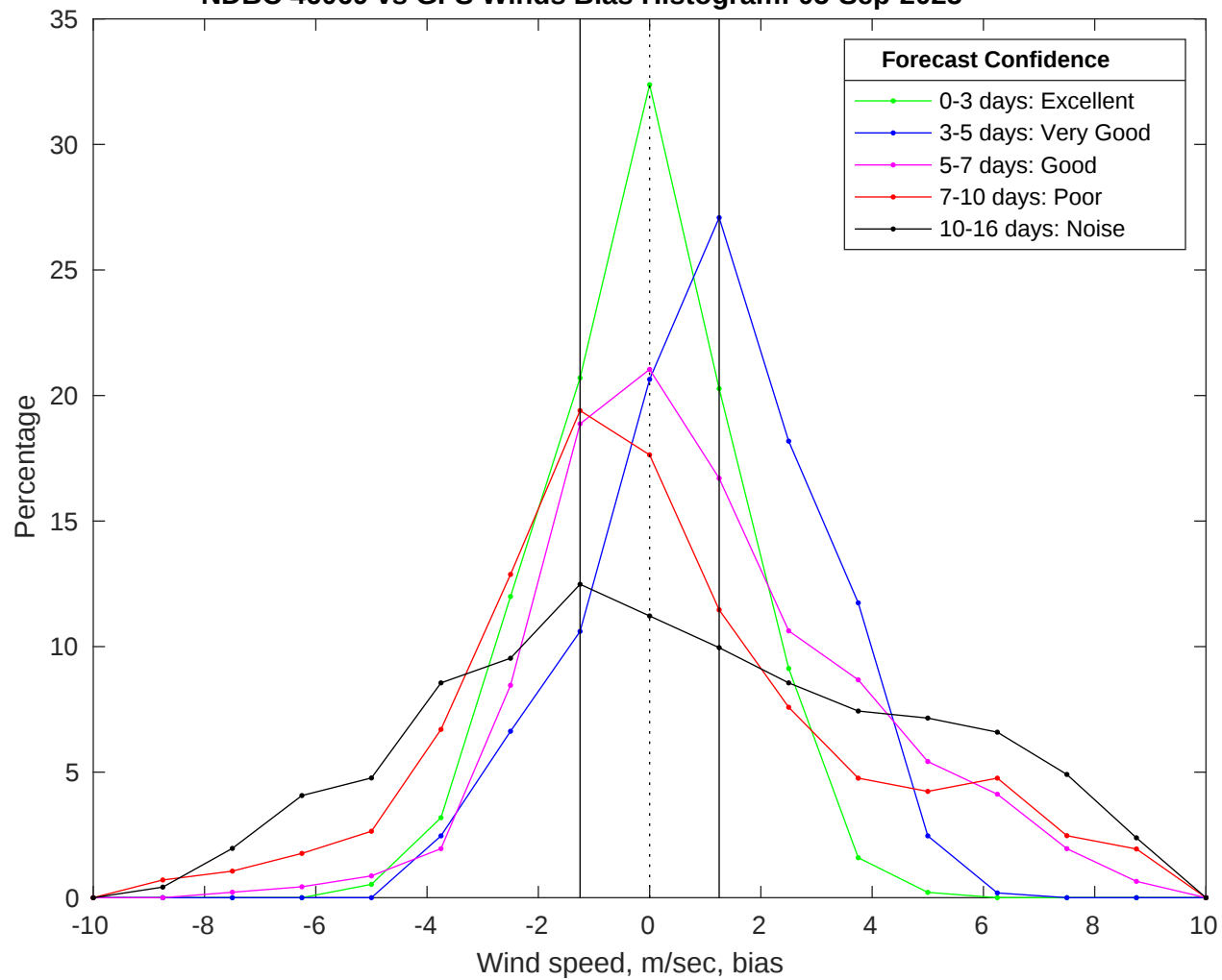
NDBC 46069 vs GFS Winds Bias Histogram: 05-Sep-2025
